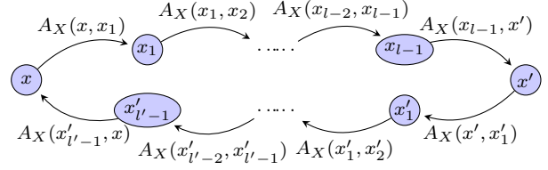
Fig. 4. Nonreciprocal clustering. Nodes x and x' are co-clustered at resolution \delta if they can be joined in both directions with possibly different (nonreciprocal) chains of maximum dissimilarity not greater than \delta [cf. (10)]. The nonreciprocal ultrametric is the smallest among all that abide to the value and transformation axioms.
