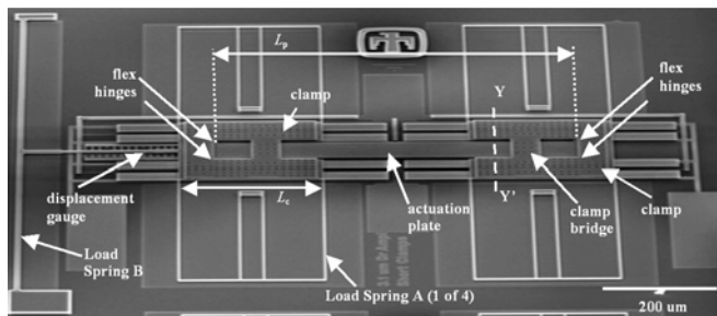
Fig. 1. An SEM image of the nanotractor friction test structure.
