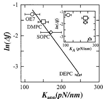
Figure 7. Correlation between membrane polarity, \Delta f , and the apparent area expansion modulus, K_{\text{app}} , for membranes: lipid (above the gel transition) or OE7. The inset shows no correlation with area expansion modulus, K_A . Data for K_{\text{app}} and K_A are those of Discher et al. (ref 37) and Rawicz et al. (ref 29).
