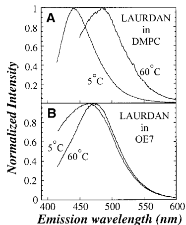
Figure 3. Emission spectra of LAURDAN in membranes of DMPC (A) and OE7 (B) when excited at 350 nm and measured at T = 5 or 60 ^{\circ}C . The emission peaks at these two temperatures were defined as \lambda_B and \lambda_R , respectively, for the calculation of generalized polarization, GP, at different temperatures. The emission spectra of LAURDAN in DMPC shows a red-shift of 40 nm from 5 to 60 ^{\circ}C , whereas LAURDAN in OE7 shows a red-shift of only 5 nm. The results indicate that the polarity of OE7 membranes does not increase significantly with temperature in comparison with DMPC membranes.
