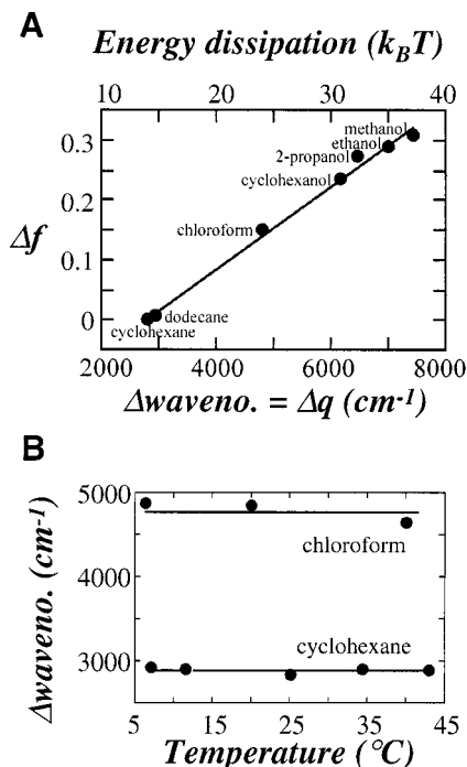
Figure 2. (A) Correlation between energy dissipation in LAURDAN fluorescence and solvent polarity. The wavenumber of the emission peak, q_{em} , is subtracted from that of the excitation peak, q_{ex} , to give \Delta q = q_{ex} - q_{em} . The polarity, \Delta f , of each solvent was calculated from its dielectric constant, \epsilon , and refractive index, n , as \Delta f = (\epsilon - 1)/(2\epsilon + 1) - (n^2 - 1)/(2n^2 + 1) (ref 6). (B) The energy dissipated from LAURDAN that is excited while dissolved in organic solvents, e.g., cyclohexane and chloroform, is essentially independent of temperature.
