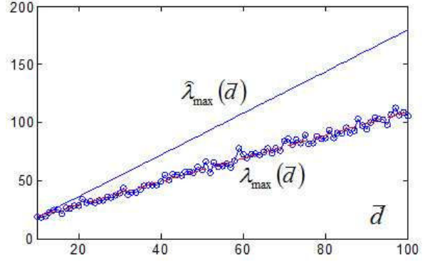
Fig. 3. Comparison between the empirical spectral radius of an RGG (circles in the plot) and the values of our analytical upper bound (solid line) for n = 1000 and r(n) = \bar{d}/2n , with expected degrees \bar{d} = [10:1:100] .
