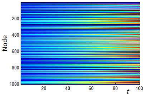
Fig. 4. Color map representing the evolution of the probabilities of infection p_i[n] for i = 1, \dots, 1000 in an RGG with n = 1000 nodes, connectivity radius r = 0.005 , rate of infection \beta = 0.020 , and recovery rate \delta = 0.018 . Each horizontal line represents the value of p_i[n] for a particular i . In this color map, blue represents a zero value, green and yellow tones represent intermediate values, and red represents values close to one. In this case, we observe an epidemic outbreak.
