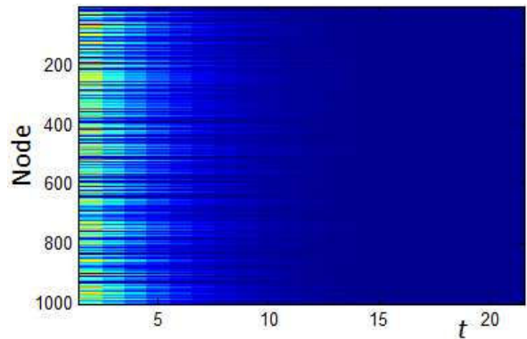
Fig. 5. Color map representing the evolution of the probabilities of infection p_i[n] when we increase the recovery rate to \delta = 0.35 (the rest of parameters are the same as we used for Fig. 5). We observe how the probability of infection of every node converges towards zero in this case.
