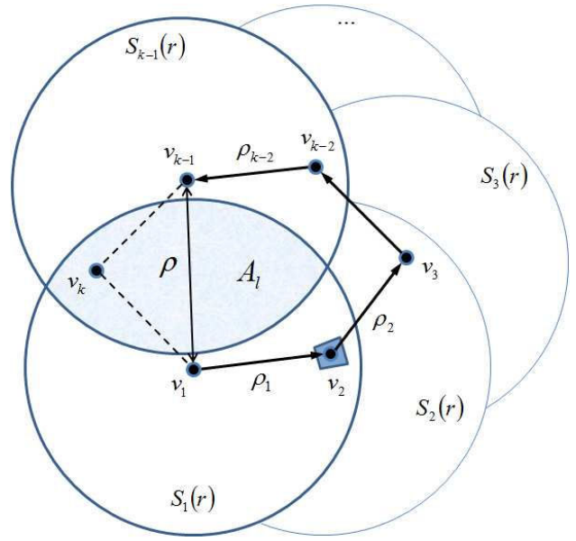
Fig. 2. This figure illustrates the technique proposed in Section III.B to count the number of closed walks of length k in a two-dimensional RGG.
