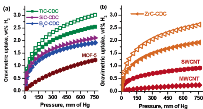
Figure 3. Hydrogen sorption isotherms. CDC produced from different carbides compared to MOF-5 (a) and nanotubes (b). Solid symbols stand for as-produced and empty for hydrogen-annealed CDC. All isotherms are completely reversible, with no hysteresis.
