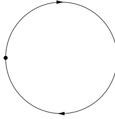
Figure 15.1: Consider a flow on a circle that moves clockwise everywhere except at a single rest point. This rest point is the unique \omega -limit point of the flow. Now suppose the flow represents the expected motion of some underlying stochastic process. If the stochastic process reaches the rest point, its expected motion is zero. Nevertheless, actual motion may occur with positive probability and in particular the process can jump past the rest point and begin another circuit. Therefore in the long run all regions of the circle are visited infinitely often. The long run behavior is captured by the notion of chain recurrence, as all points on the circle are chain recurrent under the flow.
