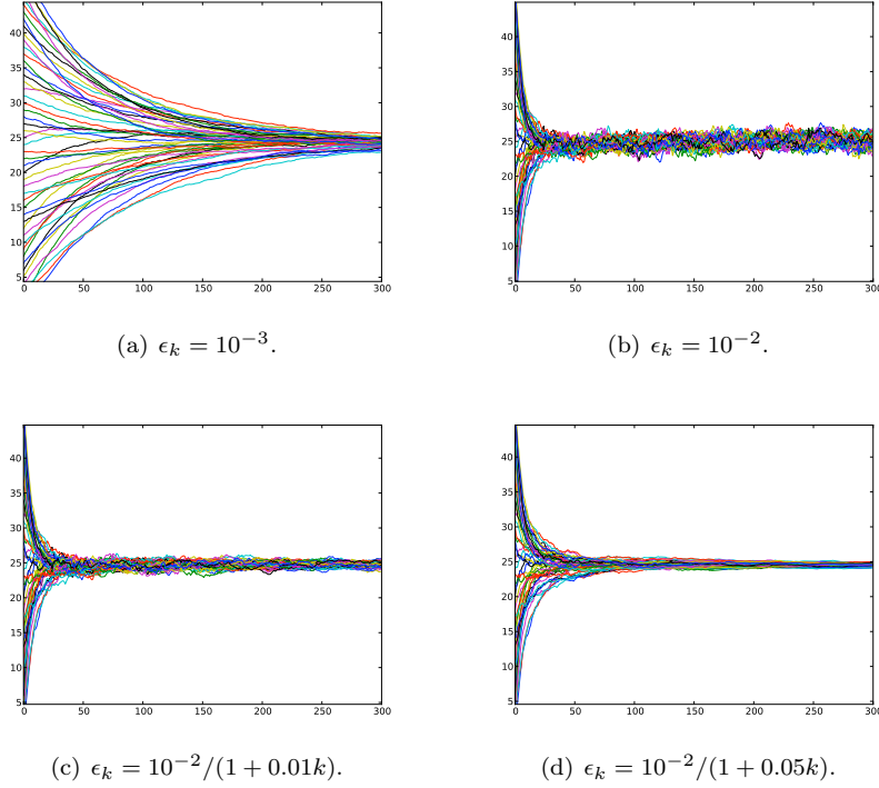
Figure 15.2: Transient behavior of the local averaging algorithm for different choices of step sizes. If we choose a constant step size, increasing it improves the convergence speed but the communication noise is not well filtered. Decreasing step sizes for larger values of k improves the asymptotic filtering property of the algorithm, but can also reduce the convergence speed if decreasing too fast. In fact for constant step sizes in this problem, we only obtain asymptotic convergence in a neighborhood of the limit set of the ODE.
