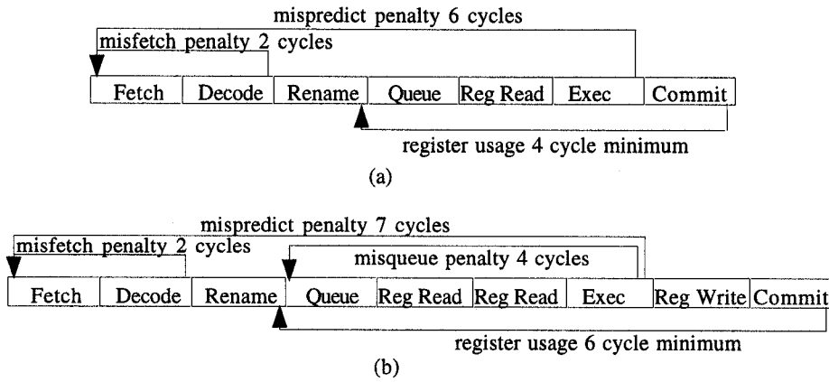
Figure 2: The pipeline of (a) a conventional superscalar processor and (b) that pipeline modified for an SMT processor, along with some implications of those pipelines.
