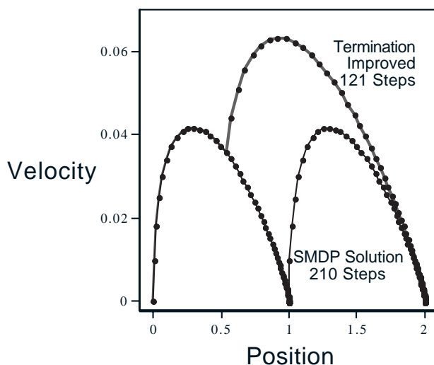
Figure 8: Phase-space plot of the SMDP and termination improved policies in a simple dynamical task. The system is a mass moving in one dimension: x_{t+1} = x_t + \dot{x}_{t+1} , \dot{x}_{t+1} = \dot{x}_t + a_t - 0.175\dot{x}_t where x_t is the position, \dot{x}_t the velocity, 0.175 a coefficient of friction, and the action a_t an applied force. Two controllers are provided as options, one that drives the position to zero velocity at x^* = 1.0 and the other to x^* = 2.0 . Whichever option is being followed at time t , its target position x^* determines the action taken, according to a_t = 0.01(x^* - x_t) .
