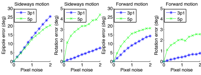
Fig. 5. Comparison of the three-plus-one algorithm with the five-point algorithm in the case when the directional constraints are derived from image points at infinity. The plots show median errors in pose estimation. The green sequences with the “x” marker show performance of the five-point algorithm and the blue sequences with the “*” marker correspond to the three-plus-one algorithm. The directional correspondences are derived from points at infinity and contaminated with the same pixel noise as the other image points. This graph shows the superior performance of the three-plus-one method in rotation estimation for forward and sideways motion, as well as translation estimation in forward motion.
