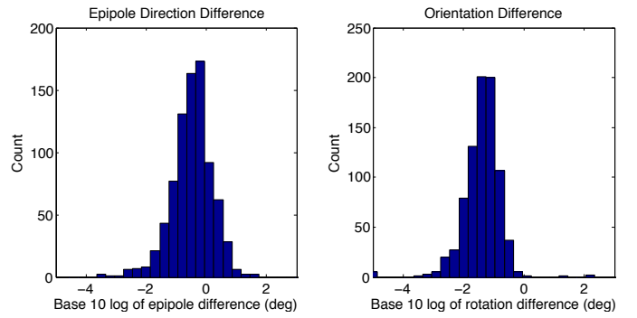
Fig. 7. Differences in recovered relative pose between our algorithm and five-point for the experiment in Figure 6. The differences are small, except the few frames where one of the methods failed to find the right hypothesis. Those places are marked on Figure 6. The differences for a total of 824 consecutive frame pairs were computed. This shows that we can count on RANSAC to choose correctly the points at infinity and that in a realistic scenario there are enough such points to enable the three plus one visual odometry.
