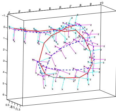
Fig. 9. Camera trajectories from a short indoor dataset where the reference direction was provided by the IMU. The red solid lines and dashed blue lines connect the centers of projection determined with our method, the five-point method, respectively. The coordinate axes attached to each point show the rig's relative orientation in space. The motion was approximately a loop, produced by hand, while exercising all six degrees of freedom, as seen by the orientation of the coordinate axis.
