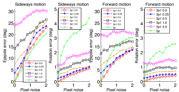
Fig. 4. Comparison of the median errors of the three-plus-one algorithm with the five-point algorithm for the cases of forward and sideways motion for different directional noise levels. In the legend, the three-plus-one algorithm is labeled “3p1”, and the five-point algorithm is labeled “5p”. The number after algorithm name indicates the standard deviation of the directional noise in degrees. The green sequence with “x” marker corresponds are the median errors in the five-point algorithm.
