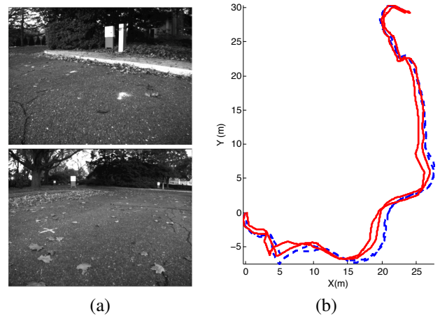
Fig. 8. (a) Sample images from the 2582-frame mobile robot data set. (b) Trajectories obtained using visual odometry with the proposed hypothesis generator and the ground truth collected using a Topcon tracking total station. The three-plus-one visual odometry (solid red) was manually scaled (with a single overall scale and a correction factor for scale drift) and aligned with the ground truth (dashed blue). The results demonstrate that the algorithm performs correctly in outdoor scenes.
