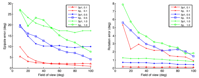
Fig. 3. Median translation and rotation errors for varying fields of view of the camera and random poses. The three-plus-one algorithm is labeled “3p1”, and the five-point algorithm is “5p”. The number after the algorithm name indicates the standard deviation of pixel and directional (for three-plus-one method only) error standard deviations levels in pixels and degrees. The colors also correspond to noise levels: red is 0.1 pixel and 0.1°, red is 0.5 pixel and 0.5°, and green is 1.0 pixel and 1.0°.
