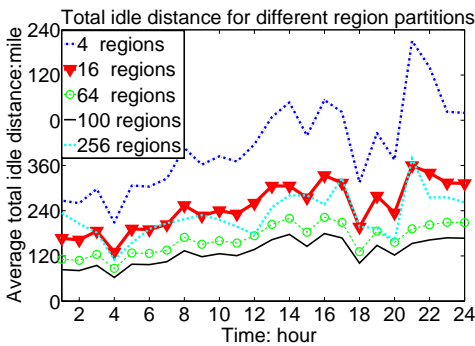
Figure 11: Average total idle distance of all taxis during one day, for different region partitions. Idle distance decreases with a larger region-division number, till the region number increases to a certain level.
