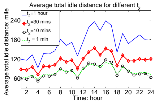
Figure 13: Comparison of average total idle distance for different t_2 – the length of time slot for updating sensor information. With a smaller t_2 , the cost is smaller. But when t_2 = 1 is too small to complete calculating problem (8), the dispatch result is not guaranteed to be better than t_2 = 10 .
