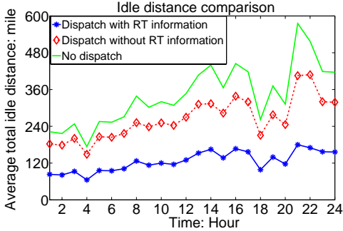
Figure 5: Average idle distance comparison for no dispatch, dispatch without real-time data, and dispatch with real-time GPS and occupancy information. Idle distance is reduced 52% given real-time information, compared with historical data without dispatch solutions.
