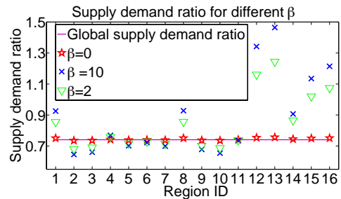
Figure 9: Comparison of supply demand ratios at each region during one time slot for different \beta values. When \beta is smaller, we put less cost weight on idle distance that taxis are allowed to run longer to some region, and taxi supply matches with the customer requests better.
