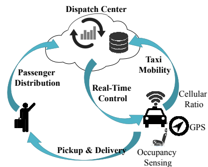
Figure 1: A prototype of the taxi dispatch system
