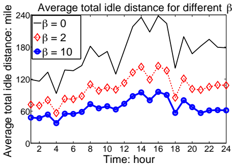
Figure 10: Average total idle distance of taxis at different hours. When \beta is larger, the idle distance cost weights more in the total cost, and the dispatch solution causes less total idle distance.
