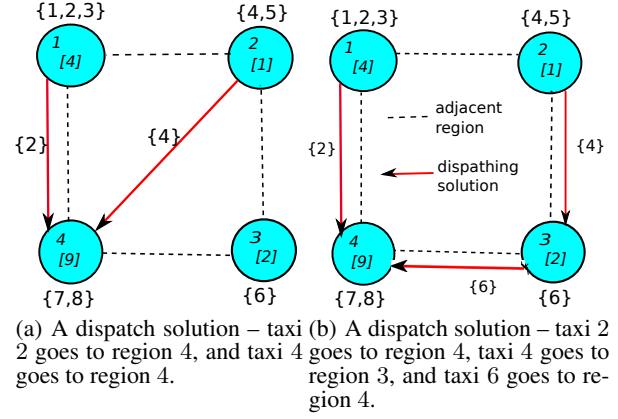
Figure 2: Unbalanced supply and demand at different regions before dispatching and possible dispatch solutions. A circle represents a region, with a number of predicted requests ( \{\cdot\} inside the circle) and vacant taxis ( \{\text{taxi IDs}\} outside the circle) before dispatching. A black dash edge means adjacent regions. A red edge with a taxi ID means sending the corresponding vacant taxi to the pointed region, to balance supply demand ratio.
