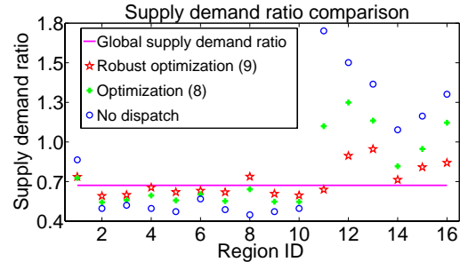
Figure 8: Comparison of supply demand ratio at each region, for solutions of robust optimization (9), problem (8) in the RHC framework, and historical data without dispatch. With the dispatch solution of problem (9), the supply demand ratio of each region is closer to the ratio of the whole city, and the total supply demand ratio error \|\frac{1}{N}\mathbf{1}_N^T X^k - \frac{1}{R^k} r^k\|_1 is reduced 46%.
