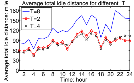
Figure 12: Average total idle distance at different time of one day compared for different prediction horizons. When T = 4 , idle distance is decreased at most hours compared with T = 2 . For T = 8 the costs are worst.
