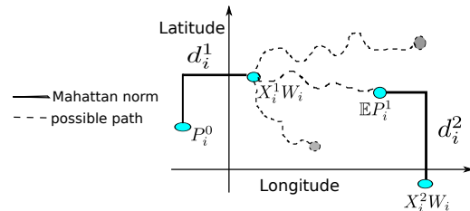
Figure 3: Illustration of a heuristic future driving distance for k = 2 : predict ending location \mathbb{E}P_i^1 in (5), get a heuristic distance to location X_i^2 W_i denoted by d_i^2 in (6).
