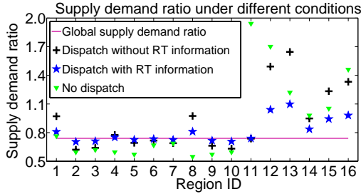
Figure 6: Supply demand ratio of the whole city and each region for different dispatch solutions. With real-time GPS and occupancy data, the supply demand ratio of each region is closest to the global level. The error of supply demand ratio \|\frac{1}{N}\mathbf{1}_N^T X^k - \frac{1}{R^k} r^k\|_1 is reduced 45% with real-time information, compared with historical data without dispatch solutions.
