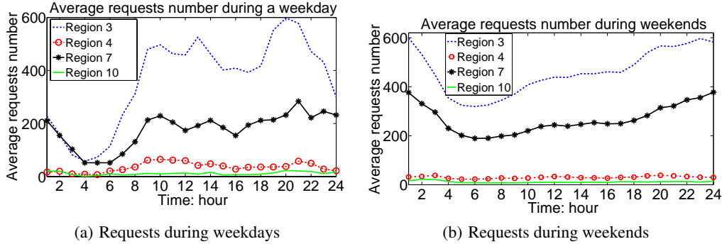
Figure 4: Requests at different hours during weekdays and weekends, for four selected regions. A given historical data set provides basic spatiotemporal information about customer demands, which we utilize with real-time data to dispatch taxis.
