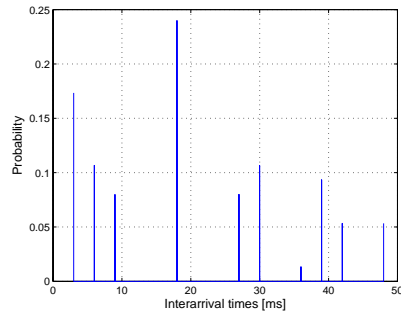
Figure 4: RT-Link PDF for 15% utilization
