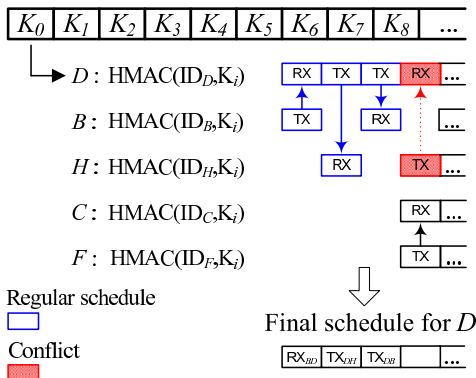
Figure 7: Implicit conflict resolution
