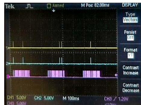
Figure 17: WisperNet-Time on Oscilloscope
