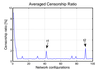
Figure 14: Averaged network's censorship ratio on 100 blocks, for implemented Steiner tree
