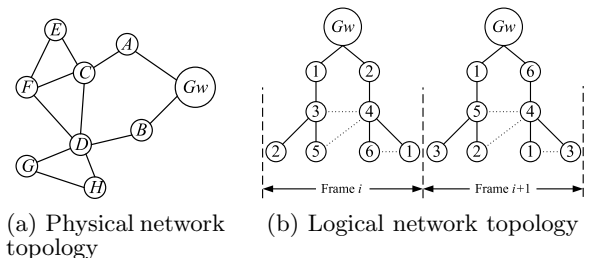
Figure 5: (a) Example network topology (b) its collision-free transmit schedule from frame-to-frame
