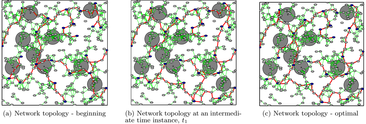
Figure 12: Network topology; green links - actual, "physical" links; red - links used for Steiner tree; blue nodes - terminal nodes (members of set L ); dark gray area - area under jammers' influence
