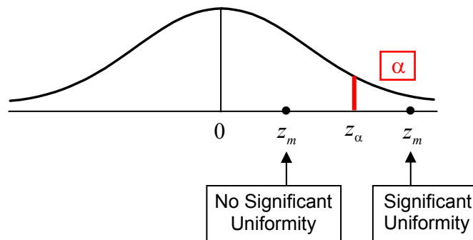
Fig.8. One-Tailed Test of Uniformity
