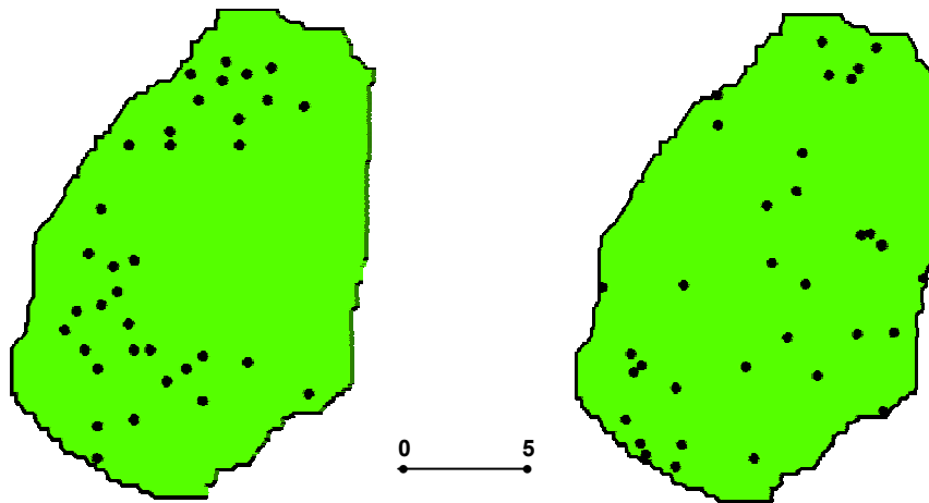
Fig.14a. Bodmin Tors
