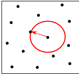
Fig.2. Uniform Pattern
