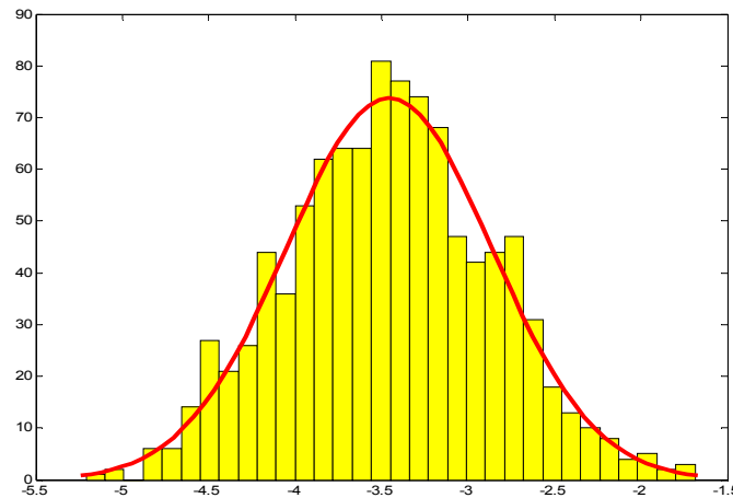
Fig.13. Sampling Distribution of Z-values
