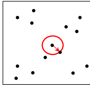
Fig.3. Clustered Pattern
