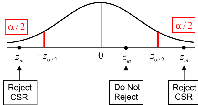
Fig.6. Two-Tailed Test of CSR
