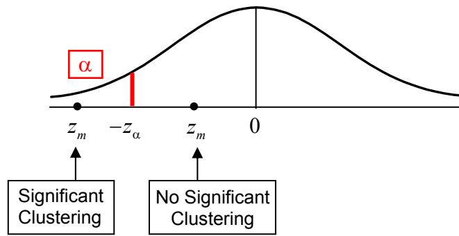
Fig.7. One-Tailed Test of Clustering
