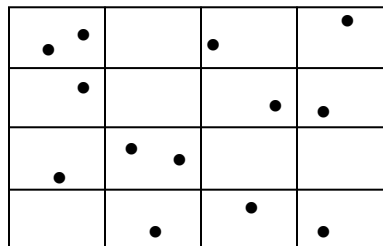
Fig. 1. Quadrat Partition of R
