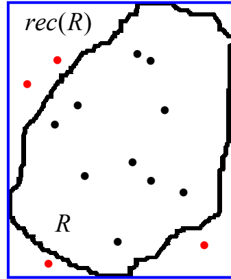
Fig.17. Rejection Sampling
