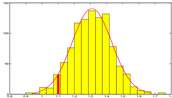
Fig.18. Histogram of Mean nn-Distances
