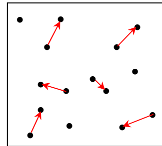
Fig.5. Independent Subset
