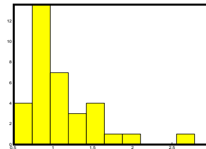
Fig.15. Bodmin nn-Distances
