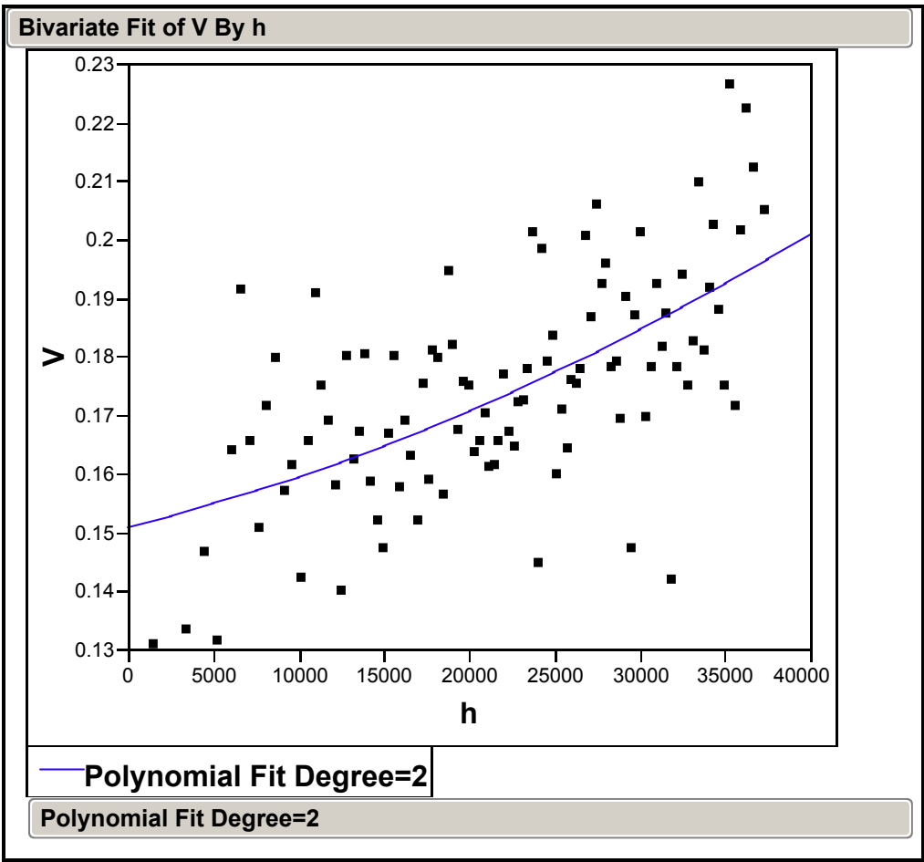
MANGANESE VARIOGRAM DATA (default bandwidth)
