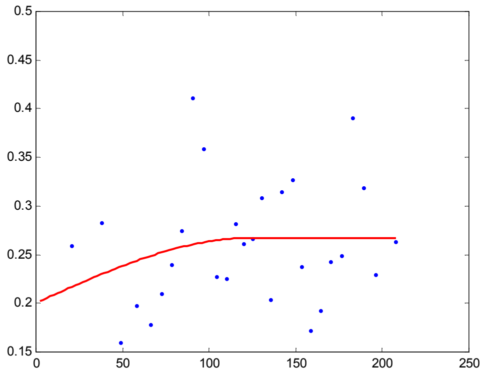
VARIOGRAM FOR ENGLAND TEMPERATURES
