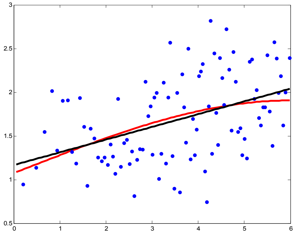
TRUNCATION OF VARIOGRAM FIT
