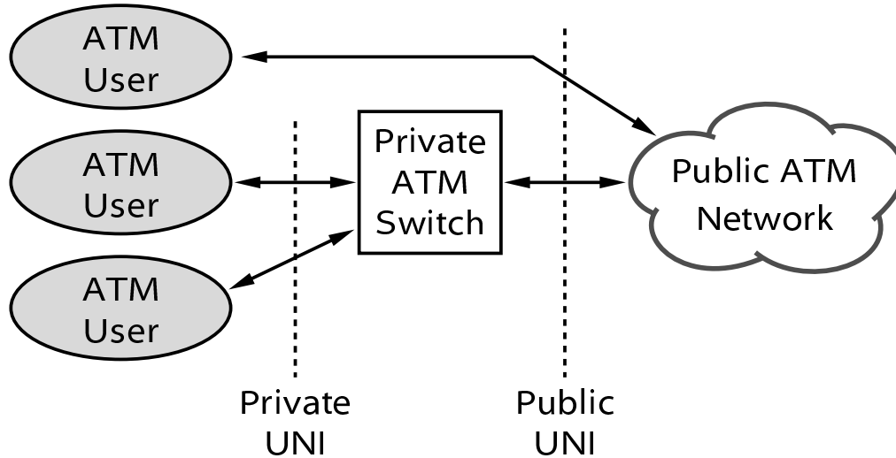
Figure 1-1 Implementations of the ATM UNI
