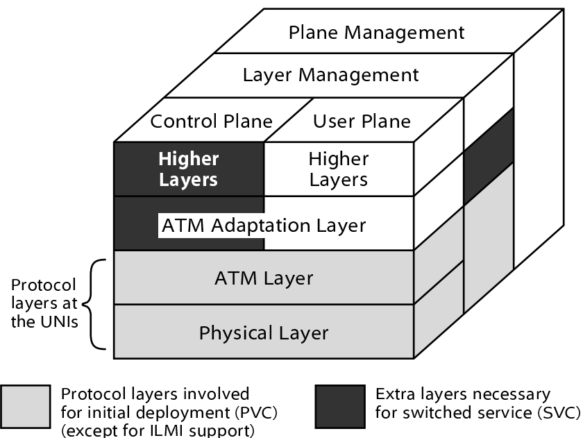
Figure 1-4 B-ISDN Protocol Reference Model
