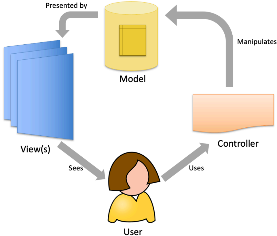
Figure 31.2: Model-View-Controller design pattern
