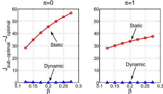
Fig. 8: Inaccurate \beta , Non-replicative.
