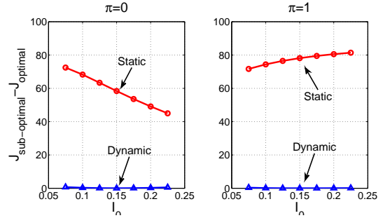
Fig. 7: Inaccurate I_0 , Replicative.
