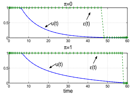
(b) Convex h(u) , Replicative
