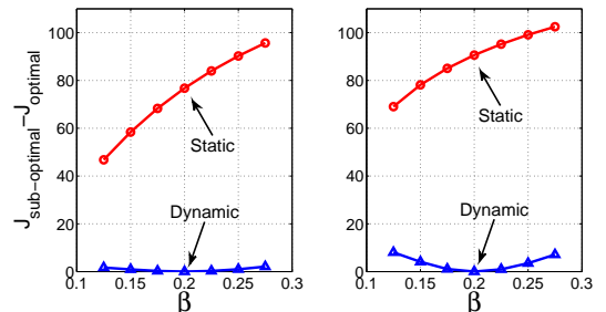
Fig. 9: Inaccurate \beta , Replicative.
