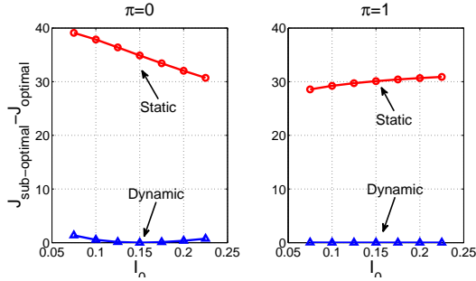
Fig. 6: Inaccurate I_0 , Non-replicative.
