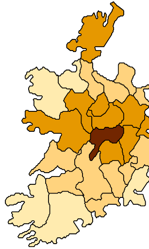
Fig.5.9. Exponential G^* -Values
