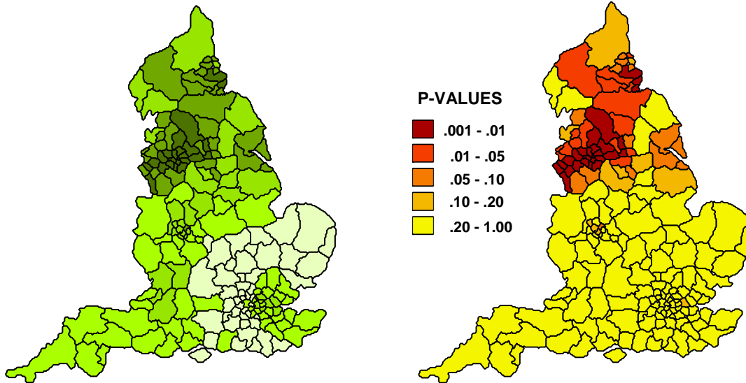
Fig.5.5. Nearest Neighbor G^* -Values
