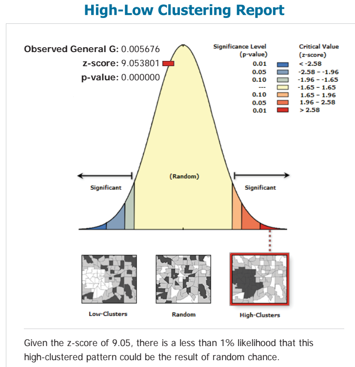
Figure 5.2. Application of the G Statistic
