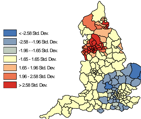
Figure 5.7. Asymptotic G^* Test Output
