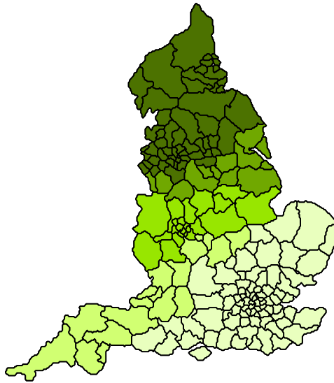
Fig.5.3. Exponential G^* -Values
