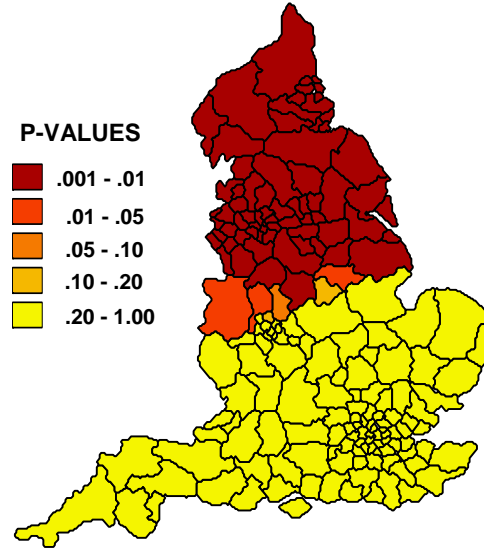
Fig.5.4. Exponential P -values
