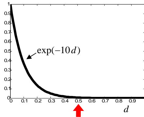
Figure 5.1. Negative Exponential Function
